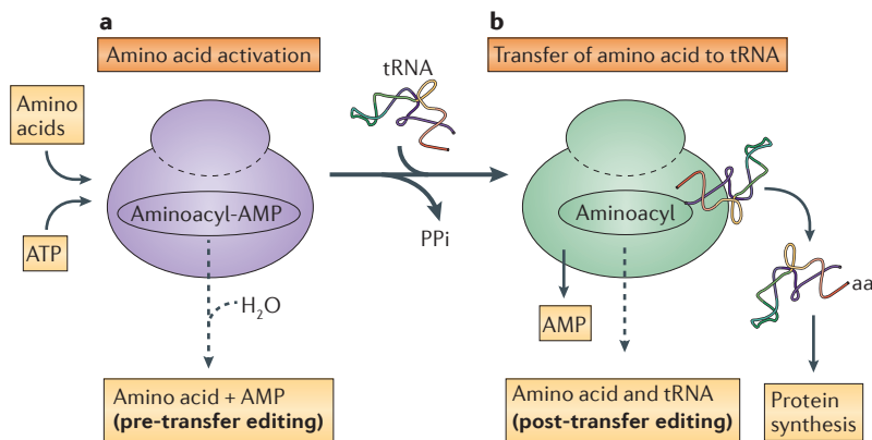
Figure 1 | Catalytic activity of ARSs. The reaction proceeds in two steps. In the first step, the substrate amino acids are activated consuming ATP (part a), and in the second step, the reaction intermediate, aminoacyladenylate (aminoacyl-AMP), is transferred to the acceptor end of tRNAs (part b). The enzymes are highly specific in substrate recognition because misrecognition of substrate amino acids or cognate tRNAs will incorporate the wrong amino acids into polypeptides. The fidelity of aminoacylation is further enhanced by proofreading that can take place before and/or after the transfer of activated amino acids to tRNAs (pre-transfer and post-transfer editing) 111 . Some aminoacyl-tRNA synthetases (ARSs) can generate diadenosine polyphosphate 112 as the secondary catalytic reaction 113 . aa, amino acids.
