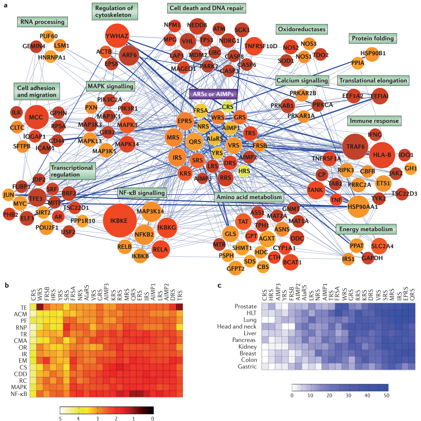
Figure 4 | Hypothetical network model showing connections of ARSs and AIMP's with their CAG interactors. a | This network model shows the links between 20 aminoacyl-tRNA synthetases (ARSs) and three ARS-interacting multi-functional proteins (AIMPs) with 123 cancer-associated genes (CAGs) (first neighbours). The network model was built with the pre-defined interactions using Cytoscape. The network nodes were arranged according to their associated GO biological process (GOBP) so that the nodes with similar GOBPs could be closely located. Nodes with multiple GOBPs are located next to the modules of GOBPs where the majority of their interactors are located (see Supplementary information S3 (text)). b | The mean shortest paths showing the close association of ARSs and AIMP's with the cellular processes represented in the network in part a are shown. Most of the ARSs and AIMP's had a low mean shortest path except for CRS, implying their close association with all the cancer pathways in the network
