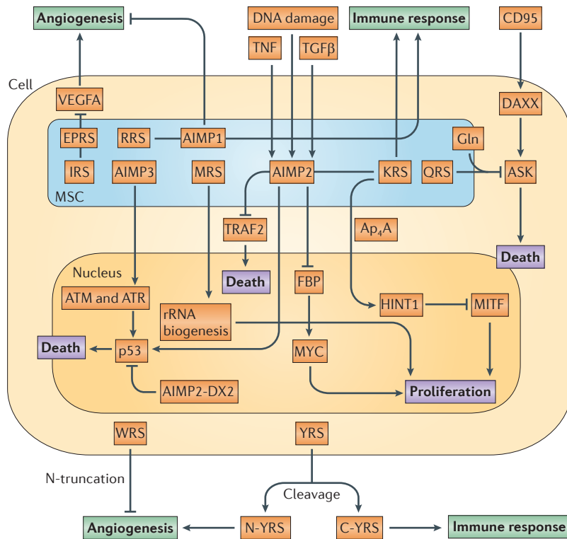
Figure 2 | Non-canonical activities of ARSs and AIMP1-3 implicated in the control of tumorigenesis. Eight different aminoacyl-tRNA synthetases (ARSs), bifunctional glutamyl-prolyl-tRNA synthetase (EPRS), isoleucyl-tRNA synthetase (IRS), leucyl-tRNA synthetase (LRS), methionyl-tRNA synthetase (MRS), glutaminyl-tRNA synthetase (QRS), lysyl-tRNA synthetase (KRS), aspartyl-tRNA synthetase (DRS) and arginyl-tRNA synthetase (RRS), form a macromolecular protein complex with three auxiliary factors, designated ARS-interacting multifunctional protein 1 (AIMP1), AIMP2 and AIMP3. This complex is known as the multisynthetase complex (MSC). Within the complex, RRS, KRS and MRS specifically interact with AIMP1, AIMP2 and AIMP3, respectively. On genotoxic damage, AIMP2 and AIMP3 are translocated to the nucleus where AIMP2 activates p53 directly 36 and AIMP3 activates p53 through the activation of the kinases ataxia telangiectasia mutated (ATM) and ATM- and Rad3-related (ATR) 40 . AIMP2 also augments the apoptotic signal of tumour necrosis factor (TNF) through downregulation of TNF receptor associated factor 2 (TRAF2) 34 and mediates the transforming growth factor- \beta (TGF \beta ) anti-proliferative signal through the downregulation of fuse-binding protein (FBP) 31 . A splice variant of AIMP2, AIMP2-DX2, compromises the tumour suppressive activity of AIMP2 and can induce tumorigenesis 39 . Among the ARSs that form the MSC, EPRS can function as a translational silencer to suppress the generation of vascular endothelial growth factor A (VEGFA), which is an angiogenic factor 53 . KRS can translocate to the nucleus to bind microphthalmia-associated transcription factor (MITF), which is an oncogenic transcriptional activator, and can generate the second catalytic product, diadenosine tetraphosphate (Ap 4 A). Ap 4 A binds a tumour suppressor histidine triad nucleotide binding protein 1 (HINT1), leading to the release of MITF, which is bound to HINT1 (REF. 114). KRS is secreted and induces the production of TNF from macrophages 69 . QRS can interact with apoptosis signal-regulating kinase 1 (ASK1) to suppress apoptotic signals in a glutamine-dependent manner 50 , and MRS can increase ribosomal RNA biogenesis in the nucleoli 48 . Among free-form ARSs, tryptophanyl-tRNA synthetase (WRS) is secreted, and the truncation of the amino-terminal peptide generates an active cytokine that suppresses angiogenesis 58 . Tyrosyl-tRNA synthetase (YRS) is also secreted and cleaved into N- and C-domains that have pro-angiogenic and immune activation functions, respectively 63 .
