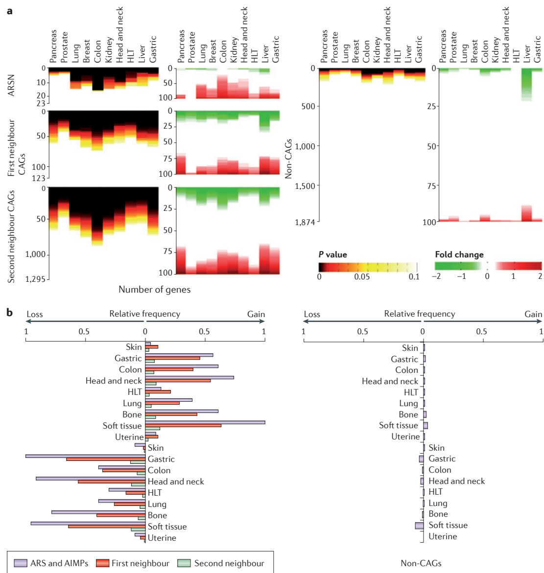
Figure 3 | Expression profiles and copy number variations of ARS-encoding genes in comparison to CAGs and non-CAGs. a | The comparison of gene expression profiles between the genes encoding 20 human cytoplasmic aminoacyl-tRNA synthetases (ARSs) and three ARS-interacting multi-functional proteins (AIMPs) (collectively termed ARSN), 123 cancer-associated genes (CAGs) that are directly linked to ARSs and AIMPs (first neighbours), 1,295 CAGs that are linked to the first ARS-neighbours (second neighbours) using the US National Cancer Institute (NCI) cancer gene index and 1,874 non-cancer associated genes (non-CAGs) is shown. Cancer-associated differential expression of each gene group was indicated by P values (left column) and fold changes (right column). The P values and the fold changes were sorted in ascending order. The P values are displayed in a red colour gradient: dark red ( P < 0.01 ), red ( 0.01 < P < 0.05 ) and white ( P > 0.05 ). The fold changes are represented by a red–green gradient showing cancer-specific increased expression and decreased expression, respectively. b | The comparison of copy number variations of ARS and AIMP-encoding genes, first, second neighbour CAGs and non-CAGs is shown. Copy number variations in the nine cancer types were obtained from the CanGEM database. For each gene group, the relative frequency of copy number variations in each cancer type is presented. HLT, haematopoietic and lymphoid tissue.
